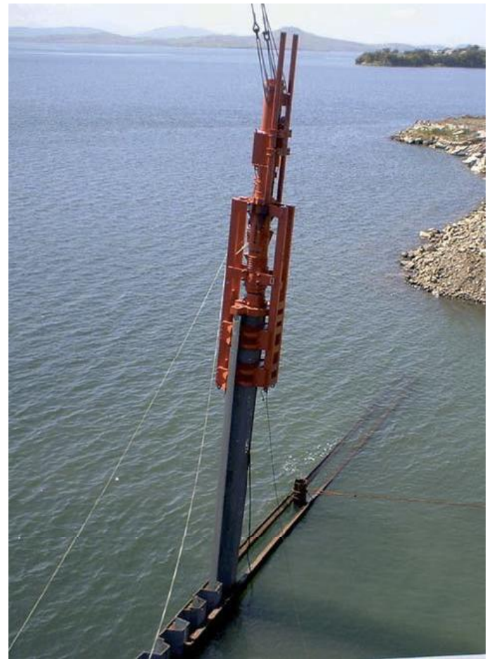
Rope suspended lead MAS 3000 with diesel pile hammer D25-32 in Russia
